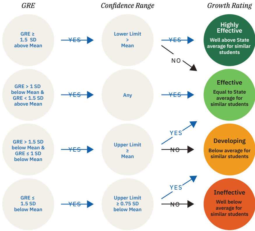
FIGURE 4. GRE CLASSIFICATION FLOWCHART
