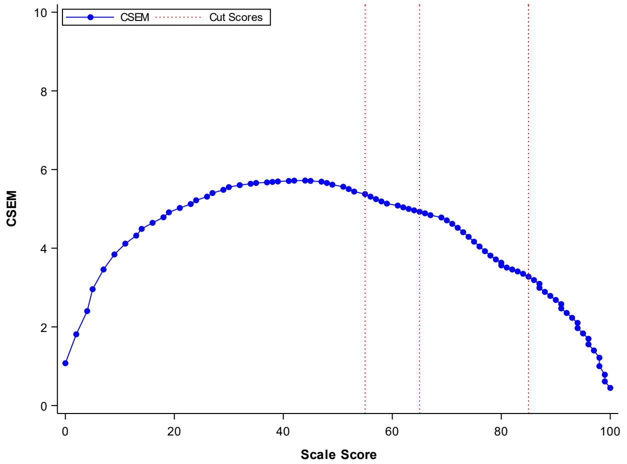
Figure E.4 Conditional Standard Error Plot: Regents Examination in Physical Setting/Earth Science
