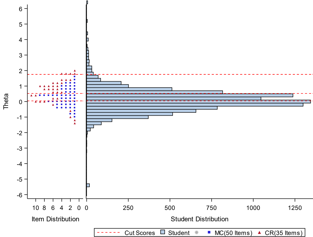
Figure D.2 Student Performance Map: Regents Examination in Physical Setting/Earth Science
