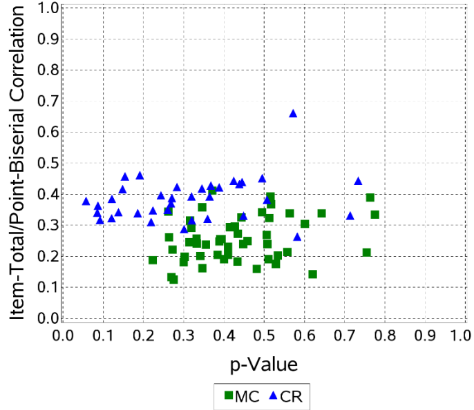
Figure E.1 Scatter Plot: Regents Examination in Physical Setting/Earth Science
