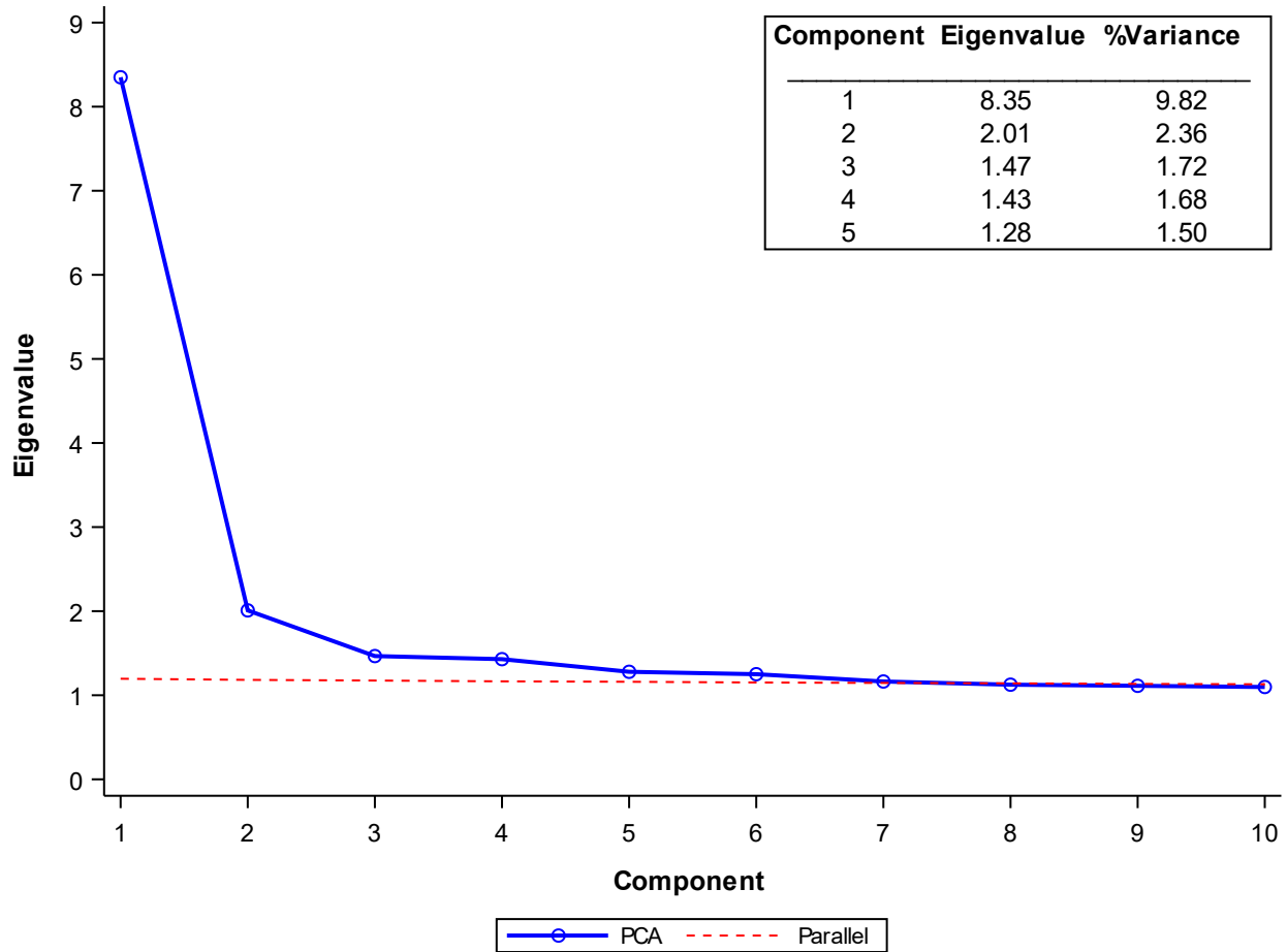
Figure D.3 Scree Plot: Regents Examination in Physical Setting/Earth Science
