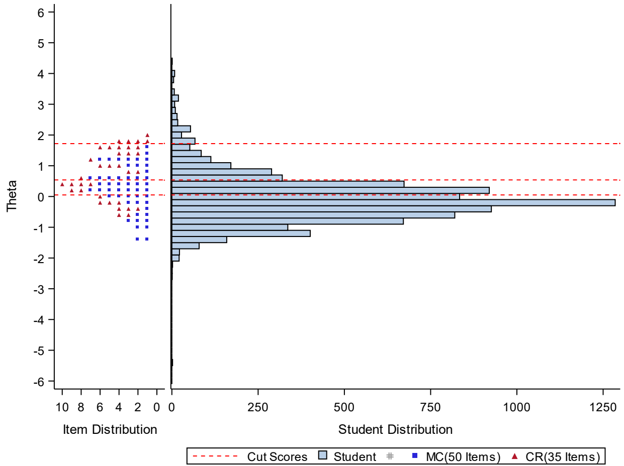
Figure E.2 Student Performance Map: Regents Examination in Physical Setting/Earth Science
