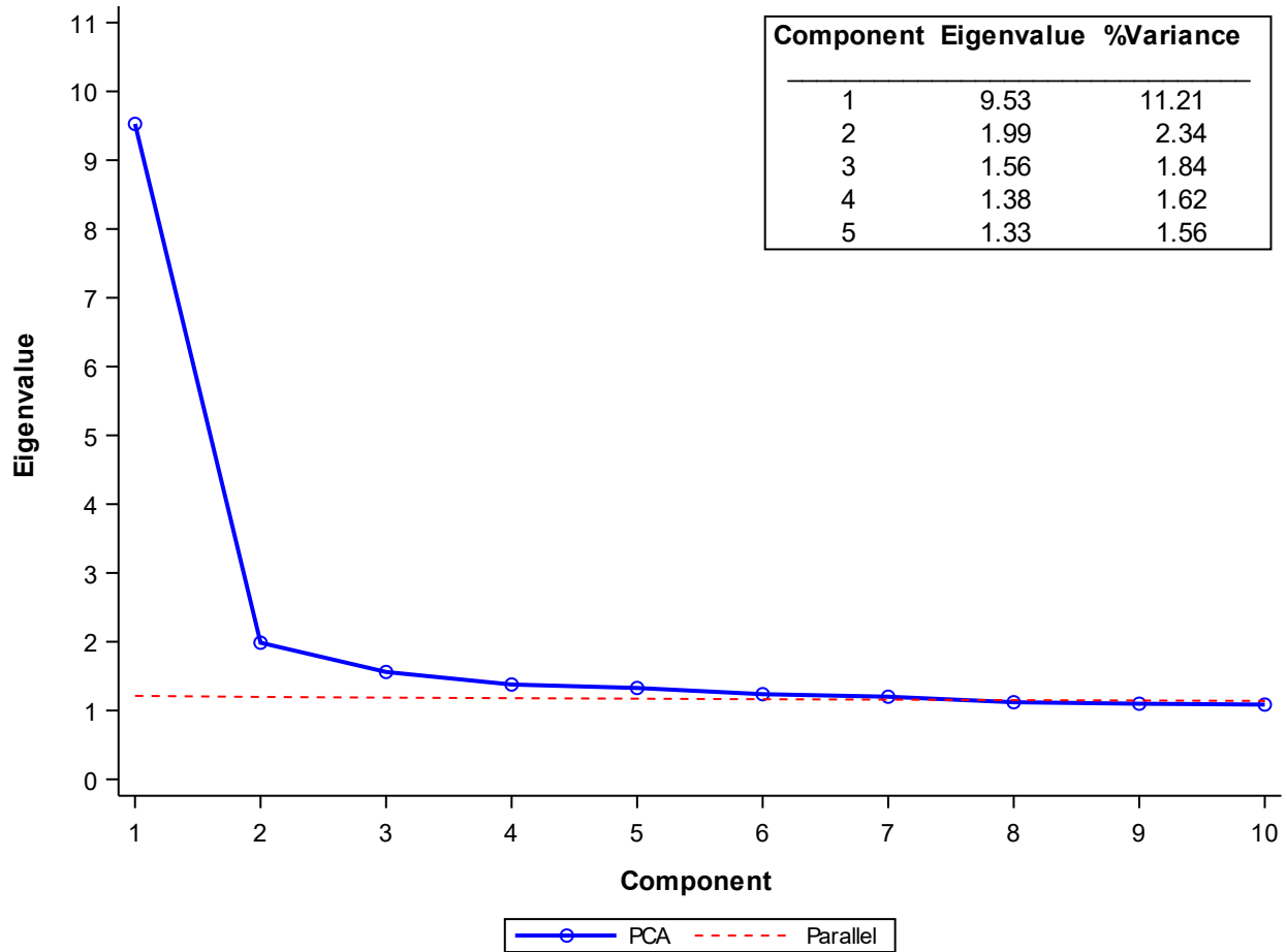
Figure E.3 Scree Plot: Regents Examination in Physical Setting/Earth Science
