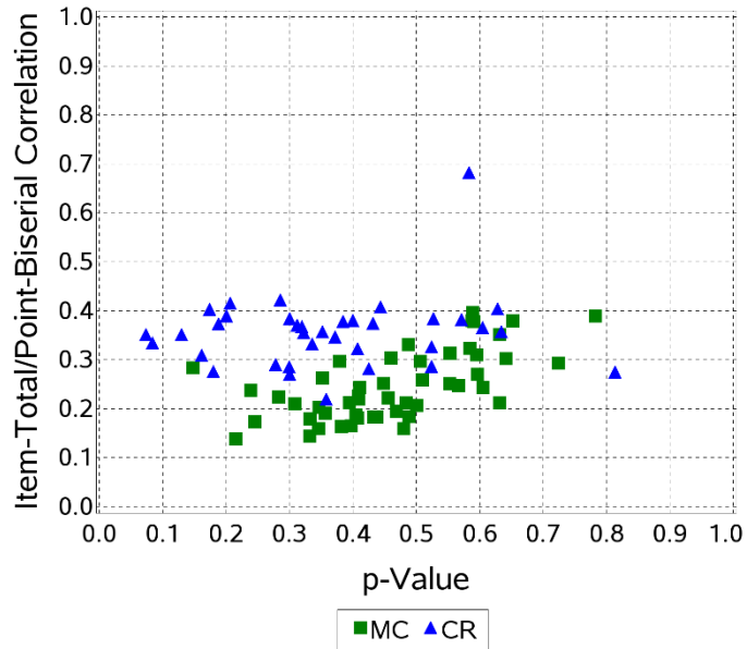
Figure D.1 Scatter Plot: Regents Examination in Physical Setting/Earth Science
