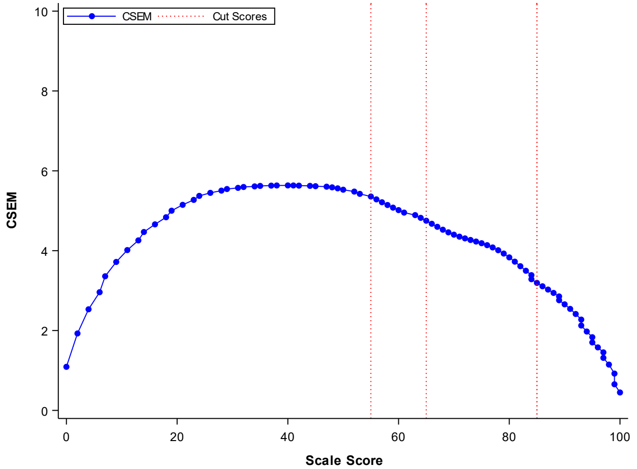
Figure D.4 Conditional Standard Error Plot: Regents Examination in Physical Setting/Earth Science
