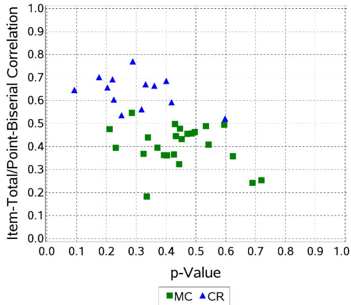
Figure E.1 Scatter Plot: Regents Examination in Algebra II
