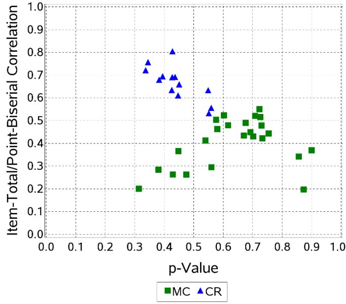
Figure 1 Scatter Plot: Regents Examination in Algebra II
