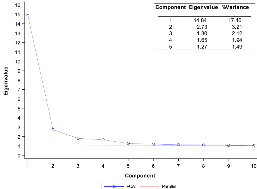
Figure 3 Scree Plot: Regents Examination in Physical Setting/Physics
