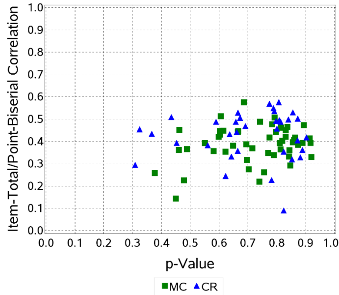
Figure 1 Scatter Plot: Regents Examination in Physical Setting/Physics
