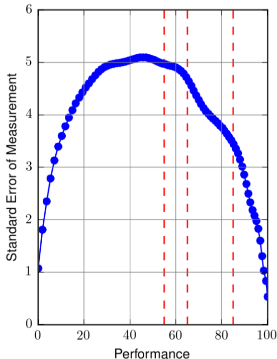
Figure 4 Conditional Standard Error Plots: Regents Examination in Physical Setting/Physics
