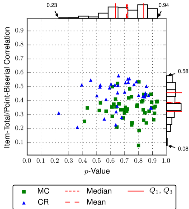
Figure 1 Scatterplot: Regents Examination in Physical Setting/Physics
