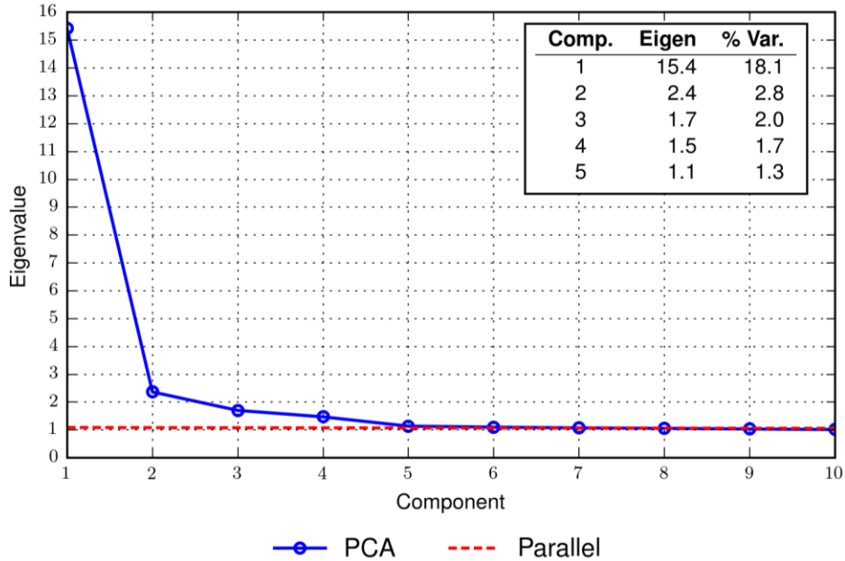
Figure 3 Scree Plots: Regents Examination in Physical Setting/Physics
