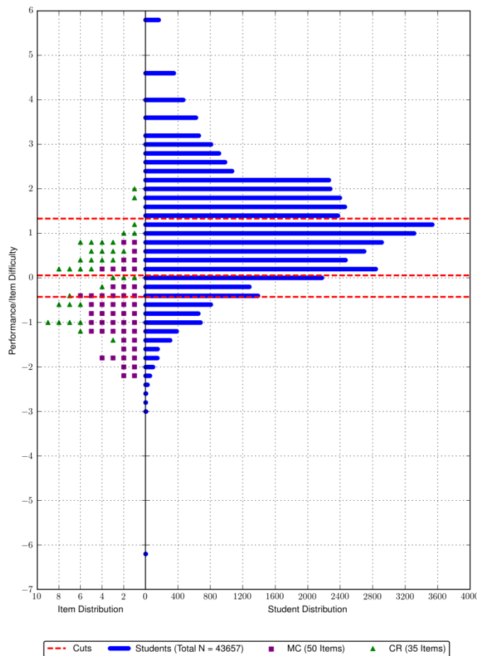
Figure 2 Student Performance Map: Regents Examination in Physical Setting/Physics
