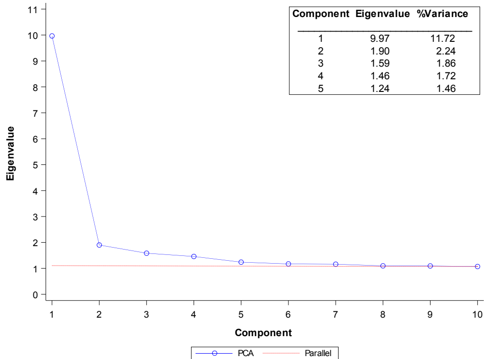
Figure E.3 Scree Plot: Regents Examination in Living Environment
