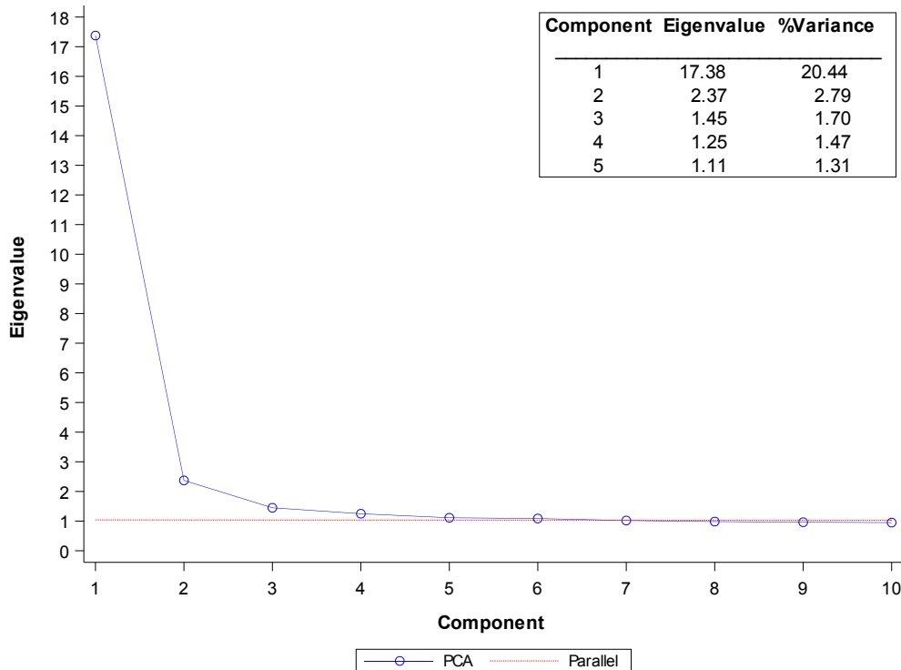
Figure 3 Scree Plot: Regents Examination in Living Environment
