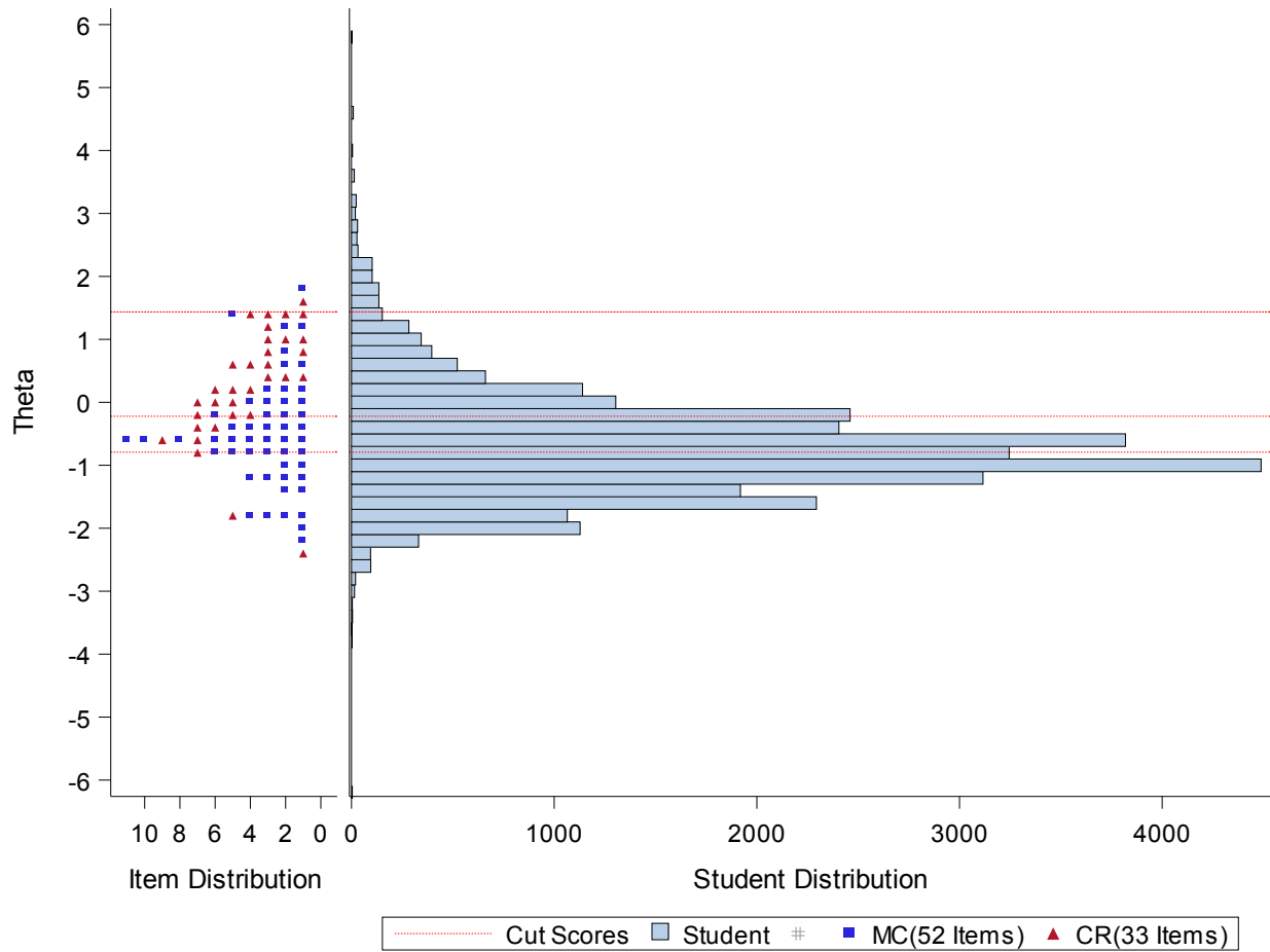
Figure E.2 Student Performance Map: Regents Examination in Living Environment
