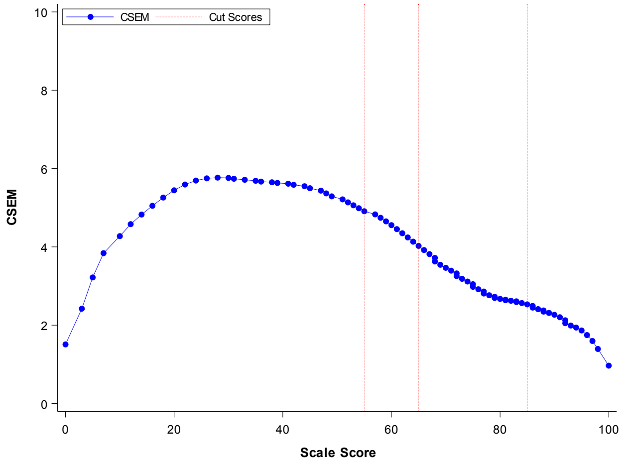
Figure D.4 Conditional Standard Error Plot: Regents Examination in Living Environment
