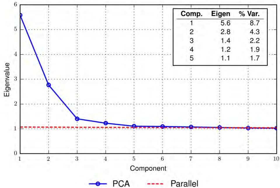
Figure C 3 Scree Plots: Regents Examination in Global History
