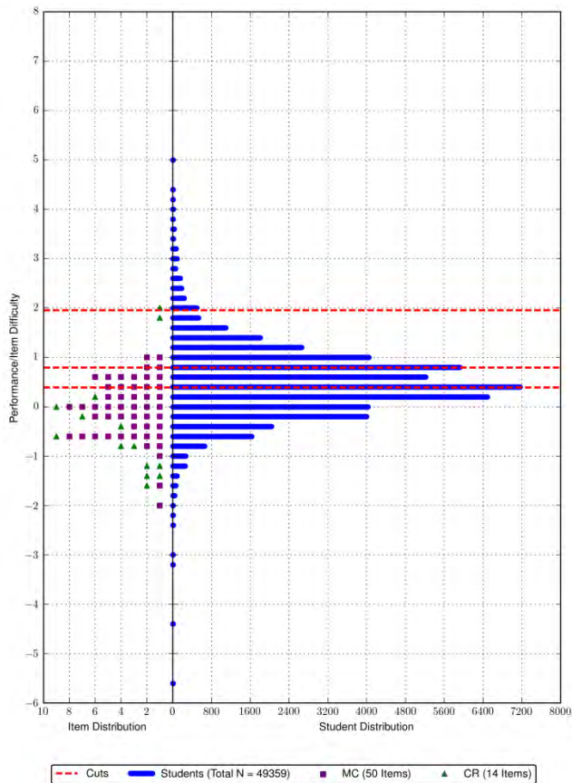
Figure C 2 Student Performance Map: Regents Examination in Global History
