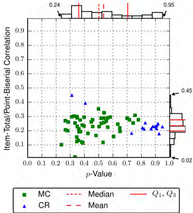
Figure C 1 Scatterplot: Regents Examination in Global History
