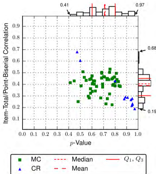
Figure 1 Scatterplot: Regents Examination in Global History
