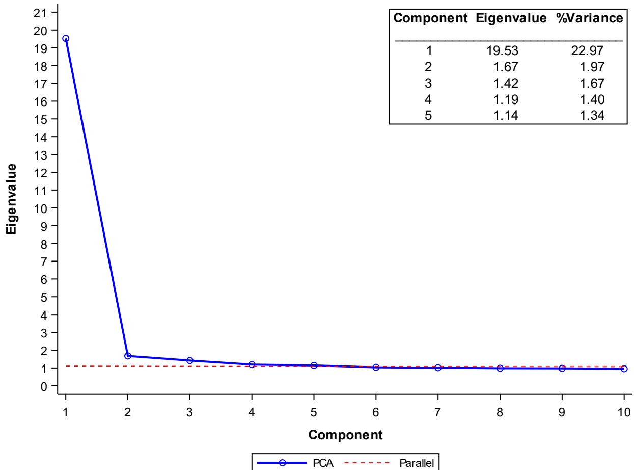
Figure 3 Scree Plot: Regents Examination in Physical Setting/Earth Science
