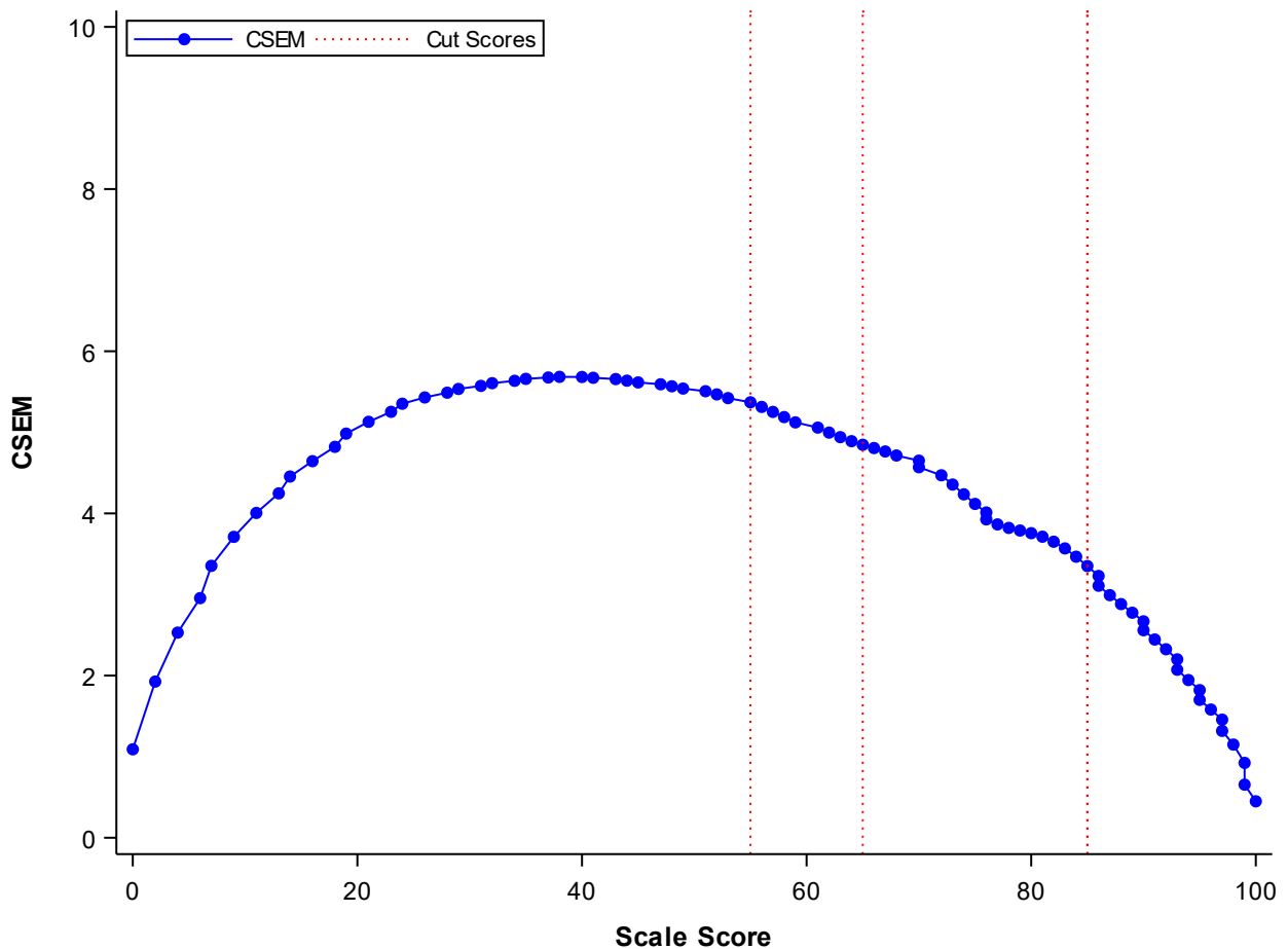
Figure 4 Conditional Standard Error Plot: Regents Examination in Physical Setting/Earth Science
