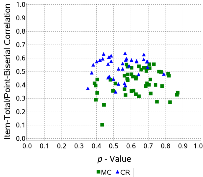
Figure 1 Scatter Plot: Regents Examination in Physical Setting/Earth Science
