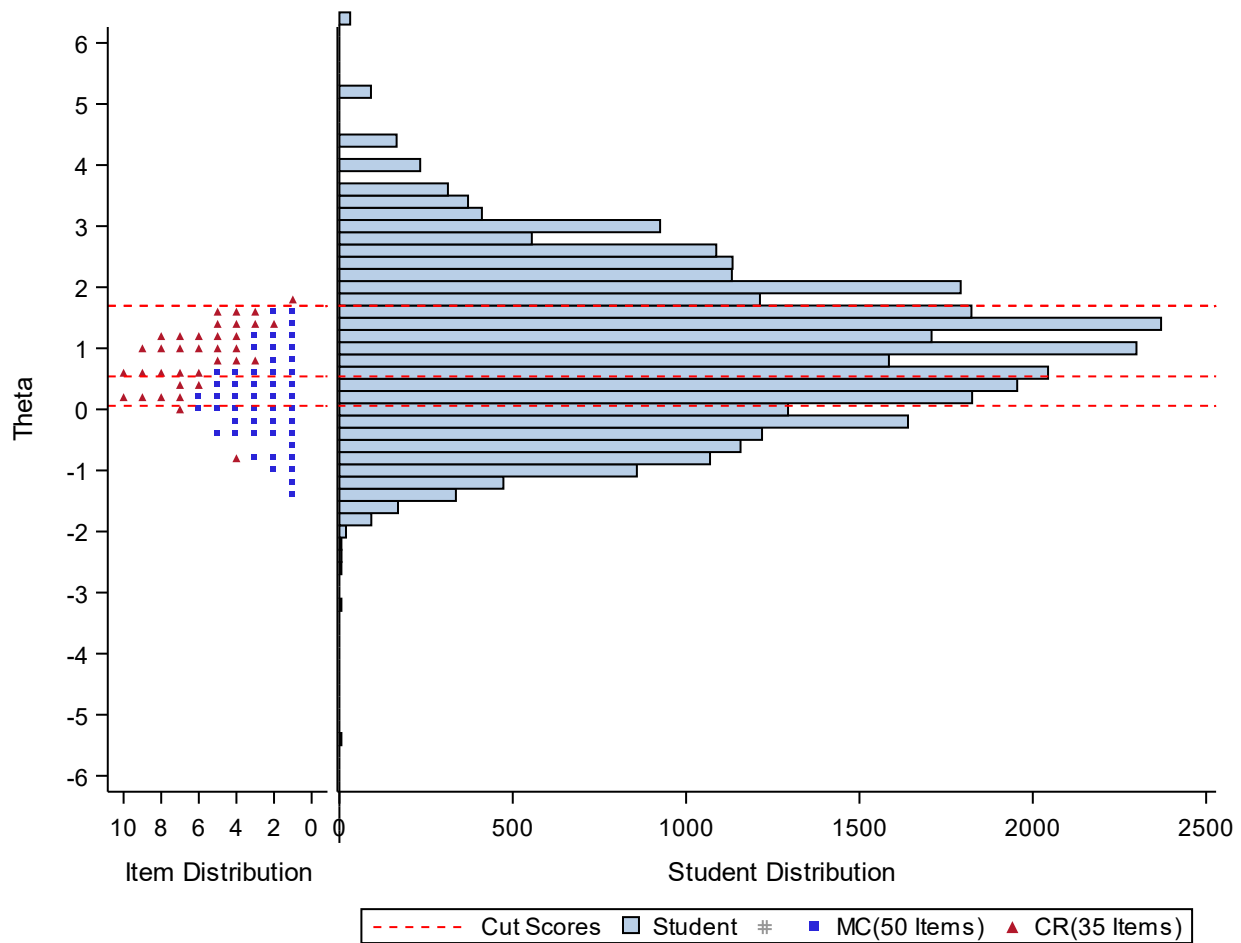
Figure 2 Student Performance Map: Regents Examination in Physical Setting/Earth Science
