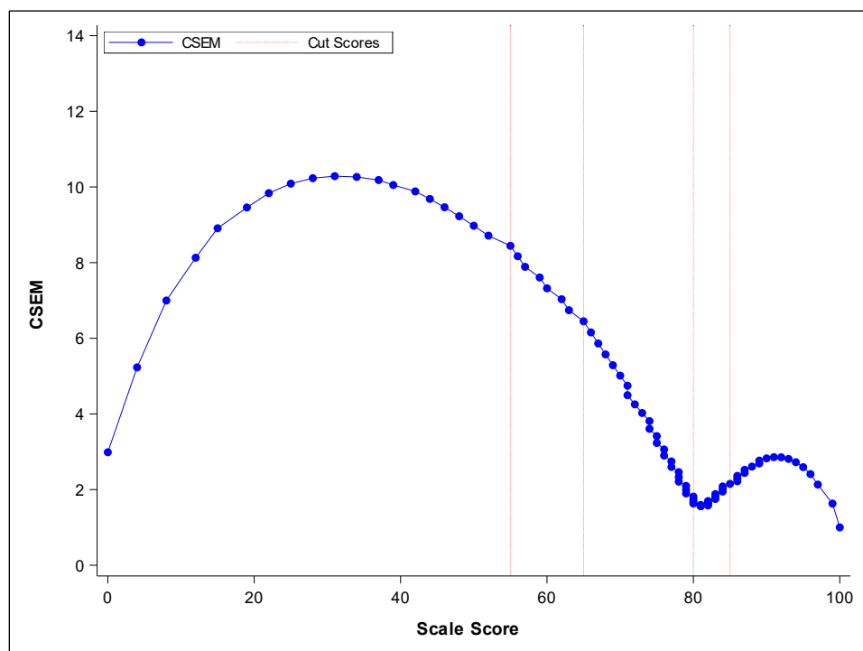
Figure E.4. Conditional Standard Error Plot: Regents Examination in Algebra I—January 2023
