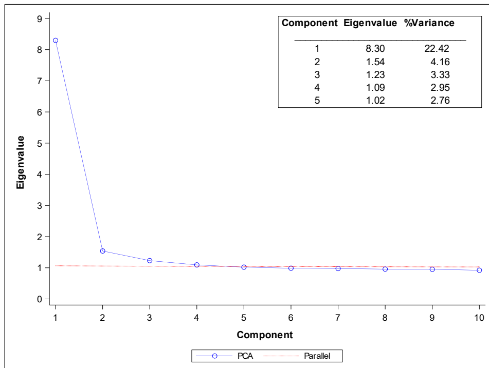
Figure E.3. Scree Plot: Regents Examination in Algebra I—January 2023
