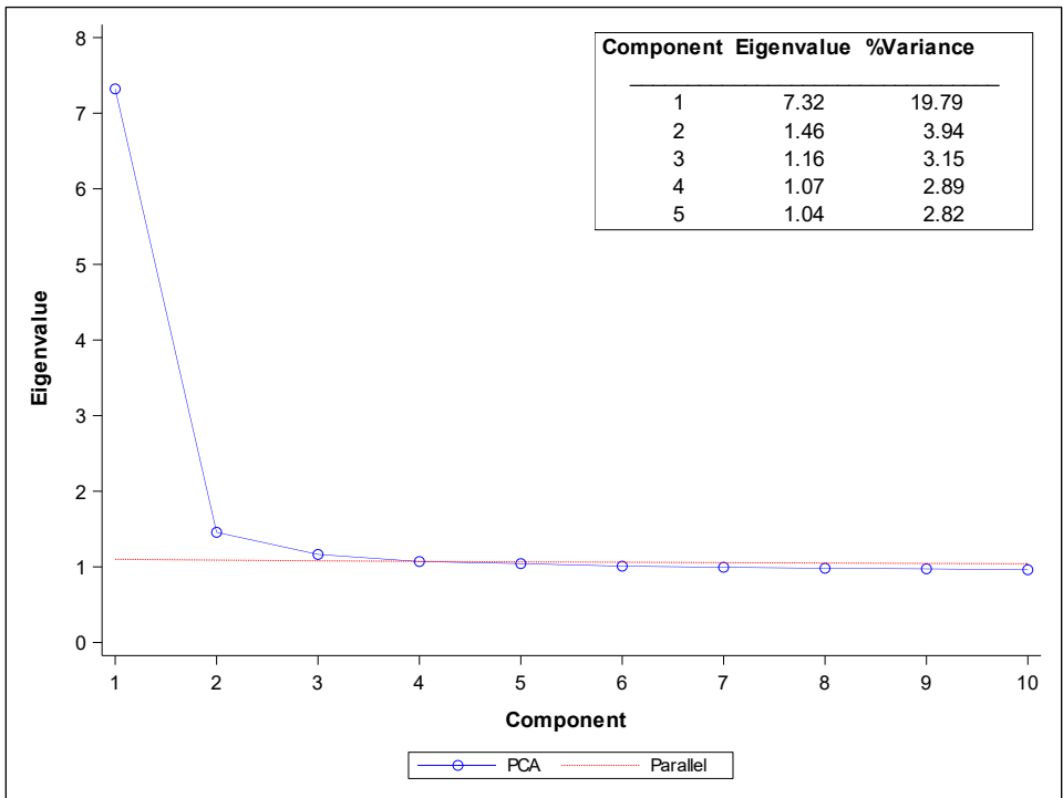
Figure D.3. Scree Plot: Regents Examination in Algebra I—August 2022
