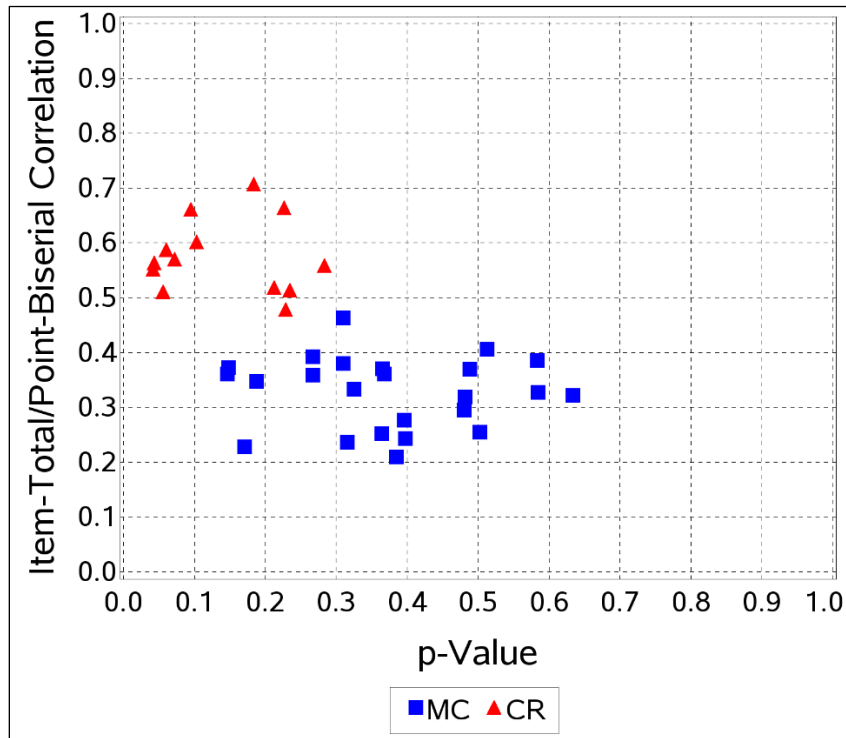
Figure D.1. Scatterplot: Regents Examination in Algebra I—August 2022
