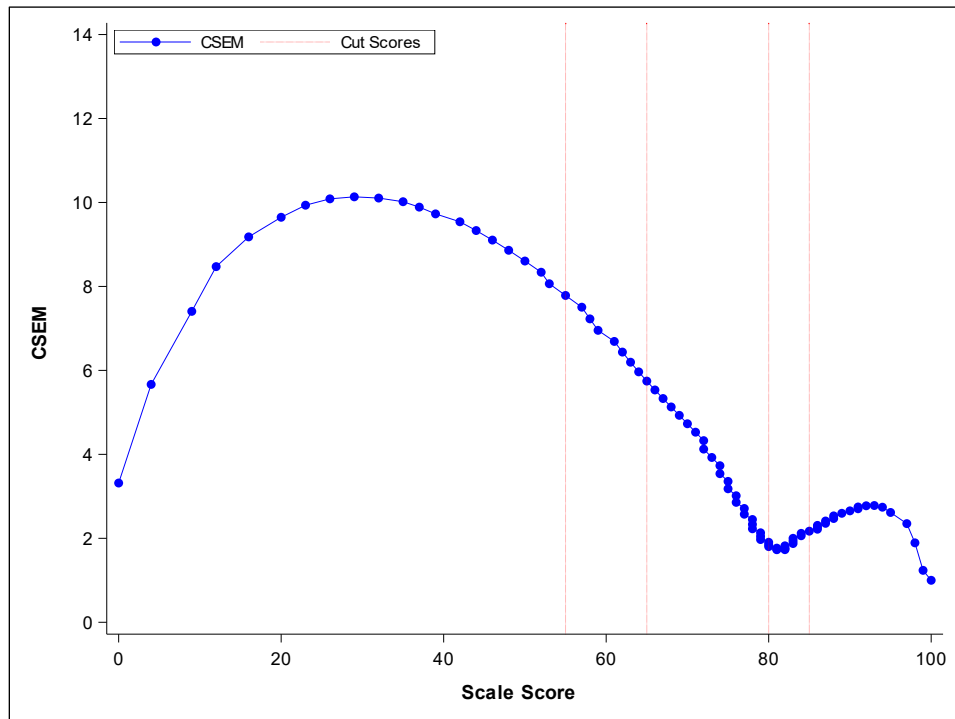
Figure D.4. Conditional Standard Error Plot: Regents Examination in Algebra I—August 2022
