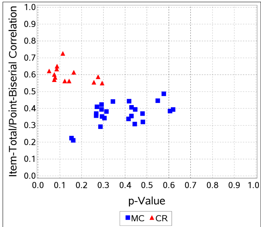
Figure E.1. Scatterplot: Regents Examination in Algebra I—January 2023
