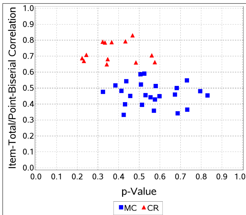
Figure 2.1. Scatterplot: Regents Examination in Algebra I—June 2023
