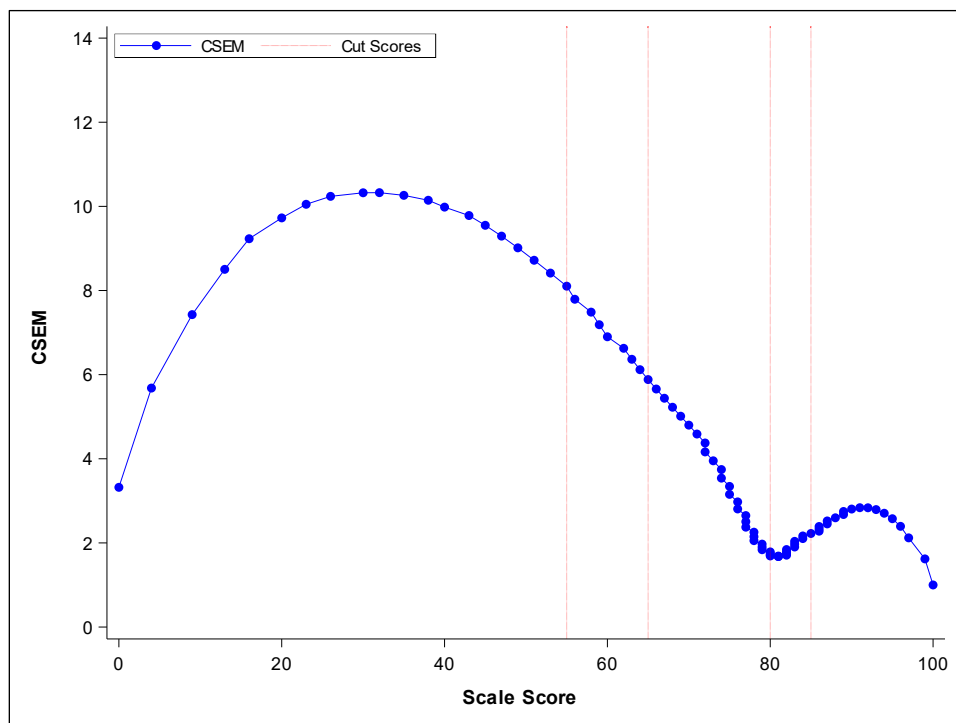
Figure 4.1. Conditional Standard Error Plot: Regents Examination in Algebra I—June 2023
