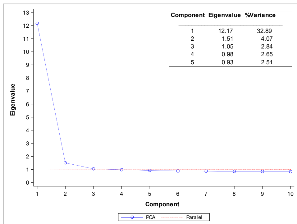
Figure 3.2. Scree Plot: Regents Examination in Algebra I—June 2023
