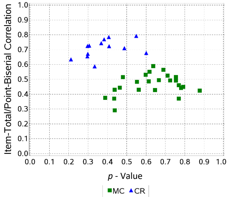
Figure 1 Scatter Plot: Regents Examination in Algebra I
