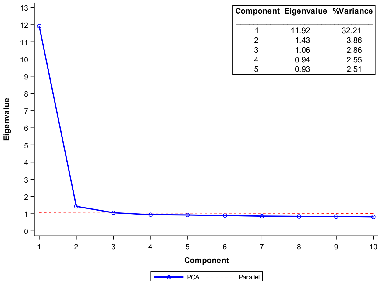
Figure 3 Scree Plot: Regents Examination in Algebra I
