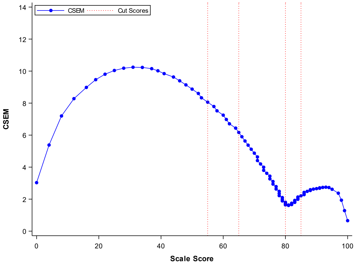
Figure 4 Conditional Standard Error Plot: Regents Examination in Algebra I
