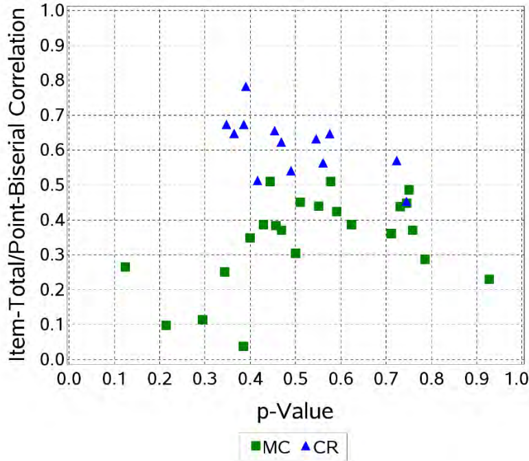
Figure 1 Scatter Plot: Regents Examination in Algebra II
