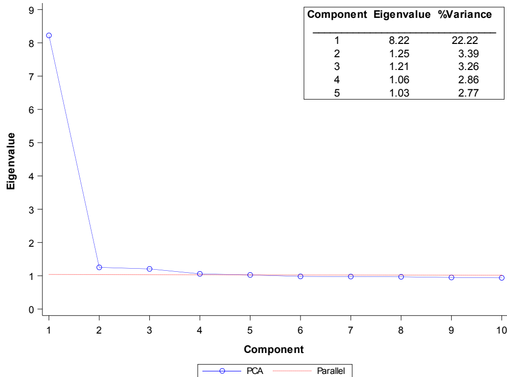
Figure 3 Scree Plot: Regents Examination in Algebra II
