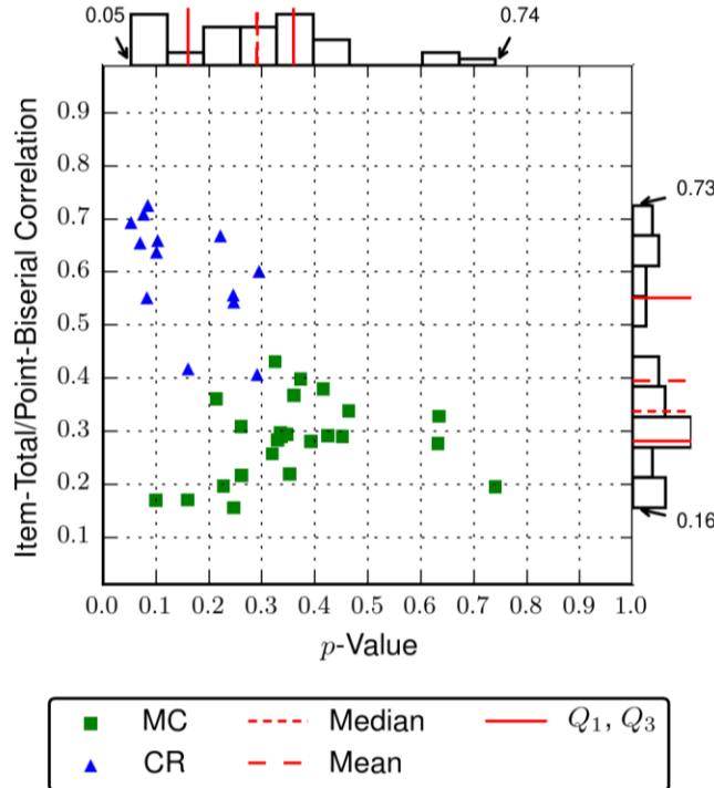
Figure B 1 Scatterplot: Regents Examination in Integrated Algebra
