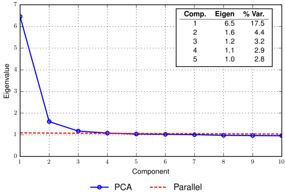
Figure C 3 Scree Plots: Regents Examination in Integrated Algebra
