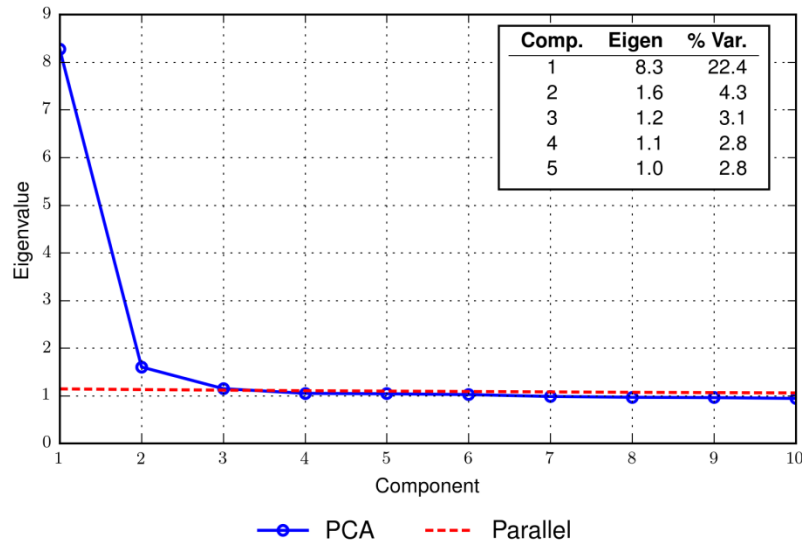
Figure B 3 Scree Plots: Regents Examination in Integrated Algebra
