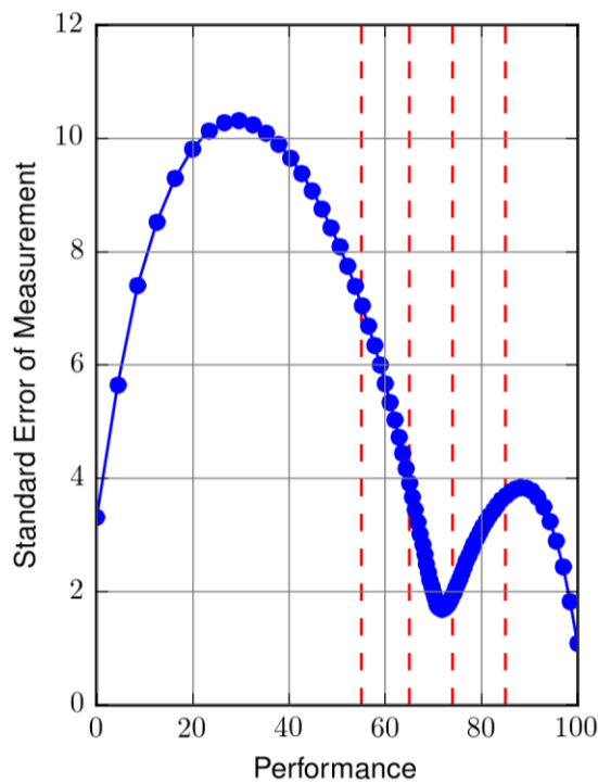
Figure C 4 Conditional Standard Error Plots: Regents Examination in Integrated Algebra
