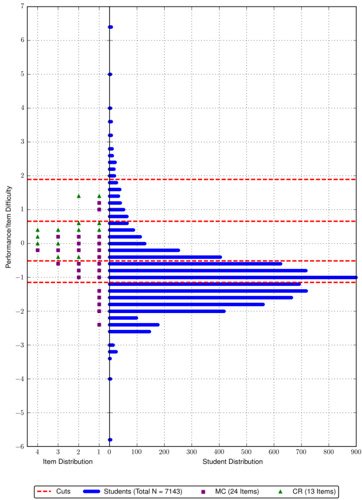
Figure B 2 Student Performance Map: Regents Examination in Integrated Algebra
