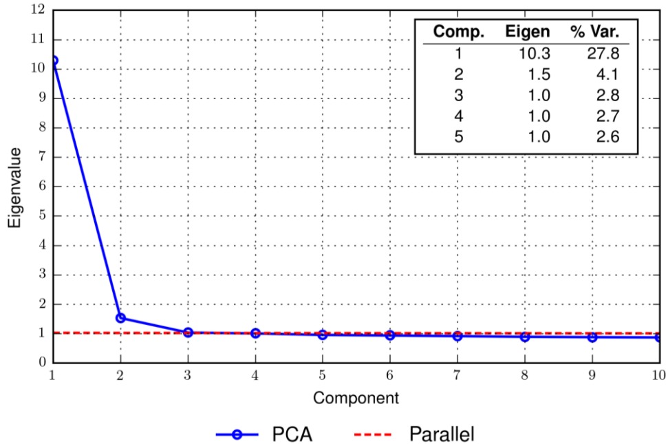
Figure 3 Scree Plots: Regents Examination in Algebra I (Common Core)
