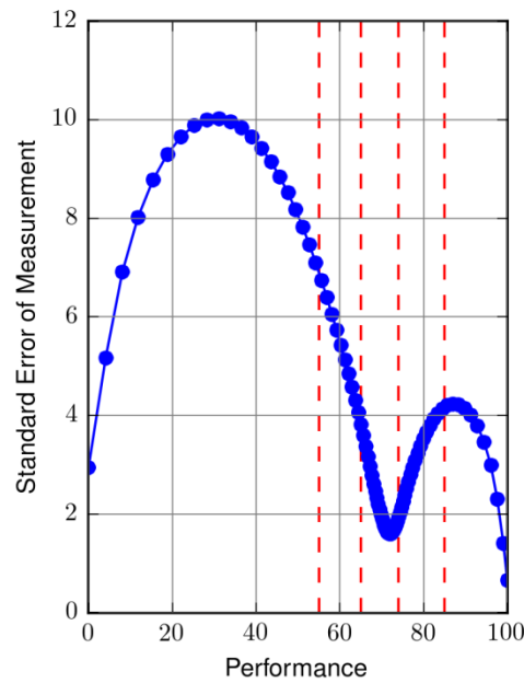
Figure B 4 Conditional Standard Error Plots: Regents Examination in Integrated Algebra
