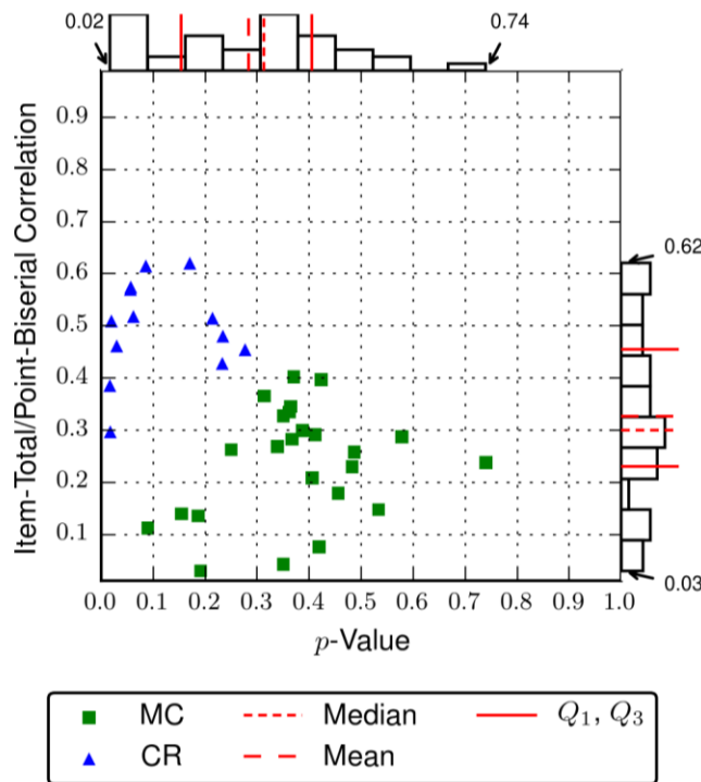
Figure C 1 Scatterplot: Regents Examination in Integrated Algebra
