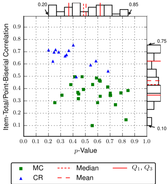
Figure 1 Scatterplot: Regents Examination in Algebra I (Common Core)
