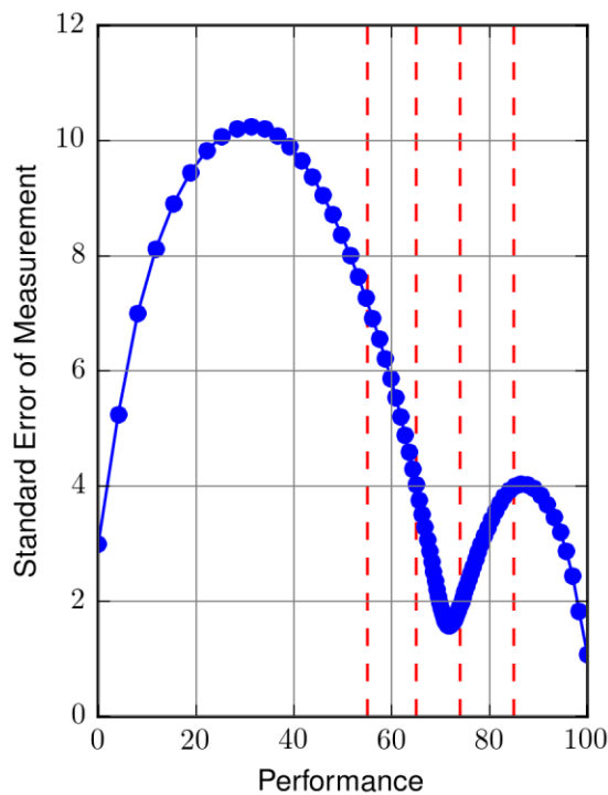
Figure 4 Conditional Standard Error Plots: Regents Examination in Algebra I (Common Core)
